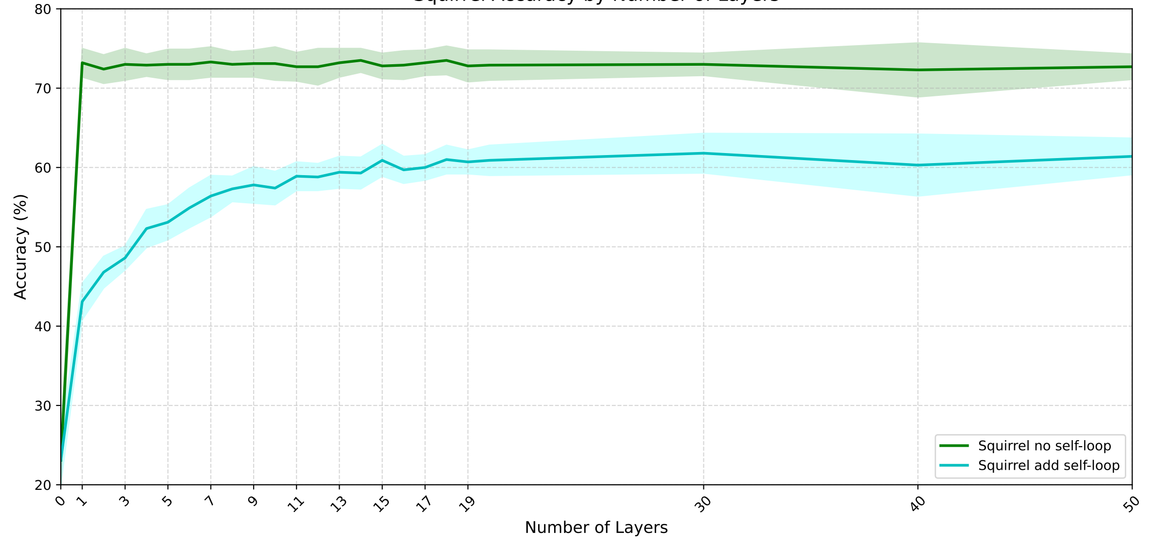
Squirrel Accuracy by Number of Layers
